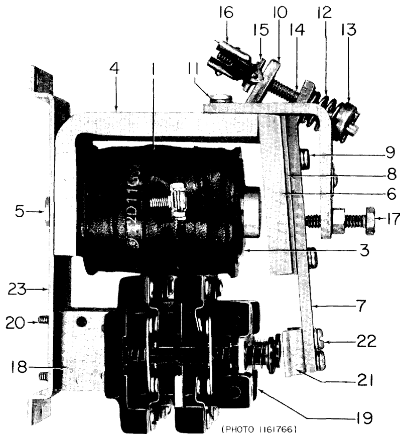
IC2820-C100B relay
